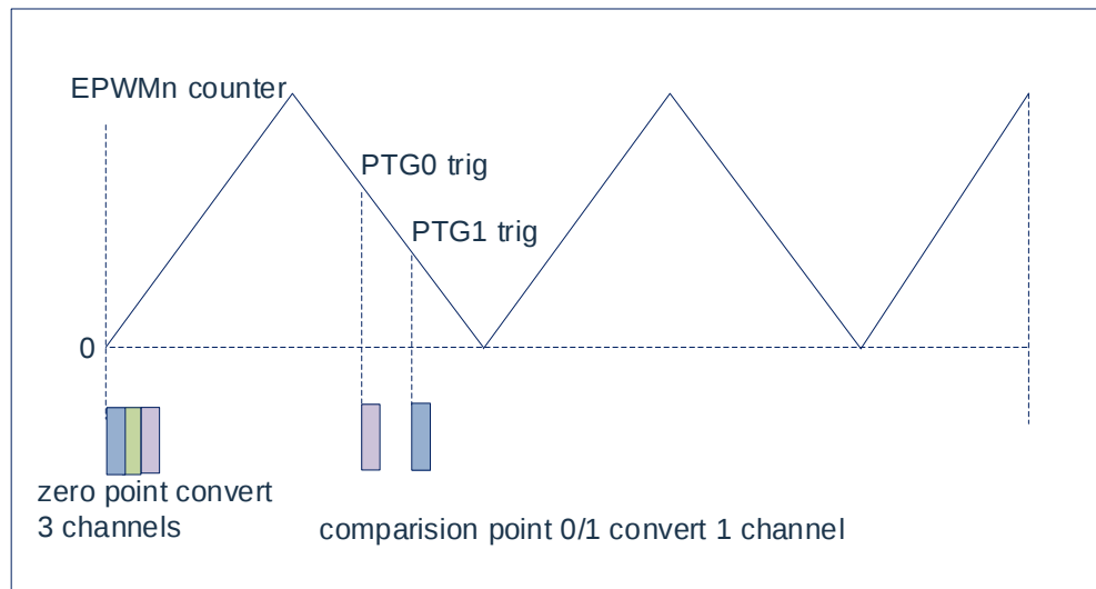
Figure 21-2: EPWM triggers to start the ADC setup
