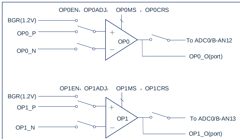
Figure 22-1: Op Amp vs. PGA Structure Diagram (1).
